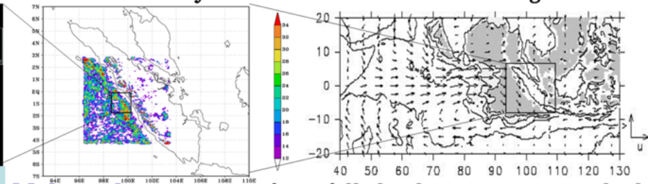
Giant diurnal cycle Observation of ISV landing over IMC
