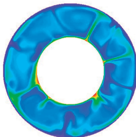
Fig. 1 The temperature field of the Rayleigh number = 10^6 .
