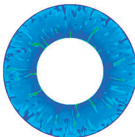
Fig. 2 The temperature field of the Rayleigh number = 10^8 .
