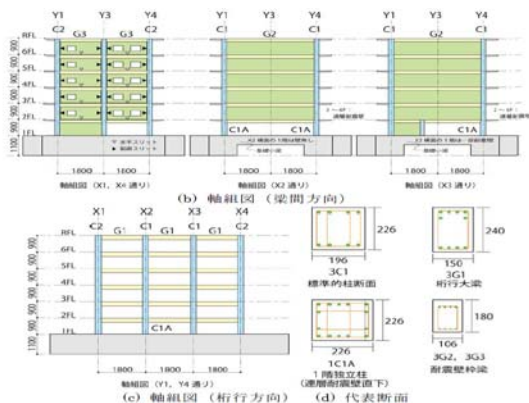
Fig. 2 Reduced model, a building with a 6-story RC shear wall frame.
